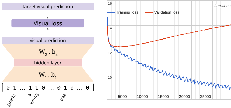
Fig. 1: Left: Architecture of a simple regressor model with one hidden layer of size 1024. Right: The training and validation loss (on y-axis) in function of the training iteration (on x-axis). Notice the model overfits in the early phase of the training process.
