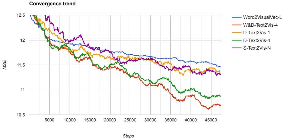
Fig. 7: Convergence error loss trends on the fc6 layer of some selected models.
