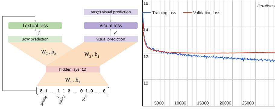
Fig. 2: Left: Architecture of our proposed S-TEXT2VIS which controls overfitting by adding an autoencoding constraint on the hidden state. Right: The training and validation loss (on y-axis) in function of the training iteration (on x-axis).
